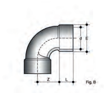
GIC 90° elbow with solvent weld sockets (fig. B)
