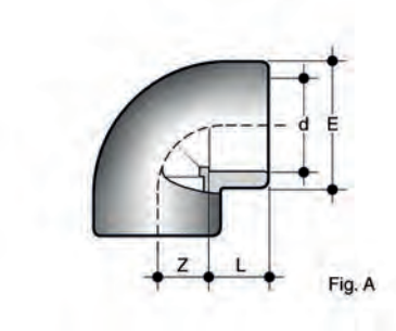
GIC 90° elbow with solvent weld sockets (fig. A)
