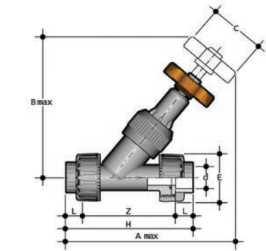
VVUIV Angle seat valve with female union ends for solvent welding, metric series
