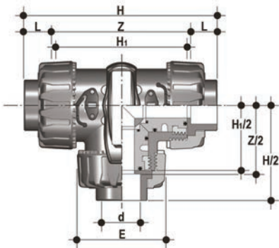
TKDIV DUAL BLOCK® 3-way ball valve with metric plain socket ends for solvent welding, T bore.
