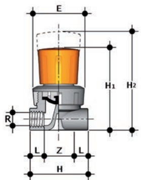
VMFV Mini-diaphragm valve with BSP threaded female ends
