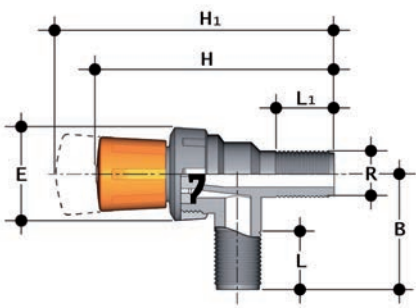
RMRV Diaphragm cock valve with BSP threaded male ends
