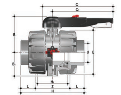
VKDLV DUAL BLOCK® 2-way ball valve with female ends for solvent welding, BS series
