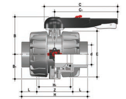
VKDIV DUAL BLOCK® 2-way ball valve with female ends, metric series
