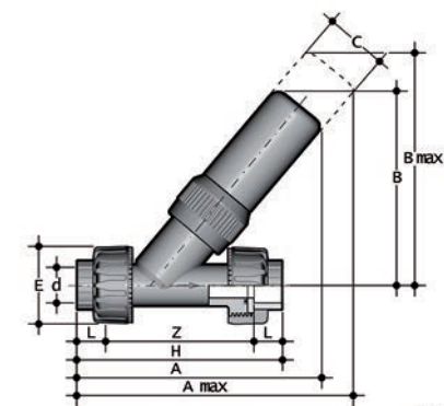
SVUIV Relief valve with unionised metric plain socket ends for solvent welding
