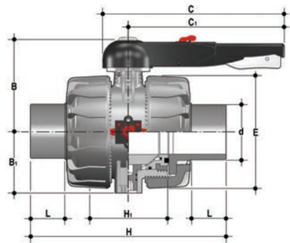
VKDDV DUAL BLOCK® 2-way ball valve with male ends for solvent welding, metric series
