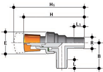
RPRV Throttling piston valve with increased flow rate, BSP threaded male ends
