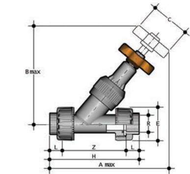
VVUFV Angle seat valve with BSP threaded female union ends
