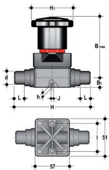
CMDV Compact diaphragm valve with male ends for solvent welding, metric series
